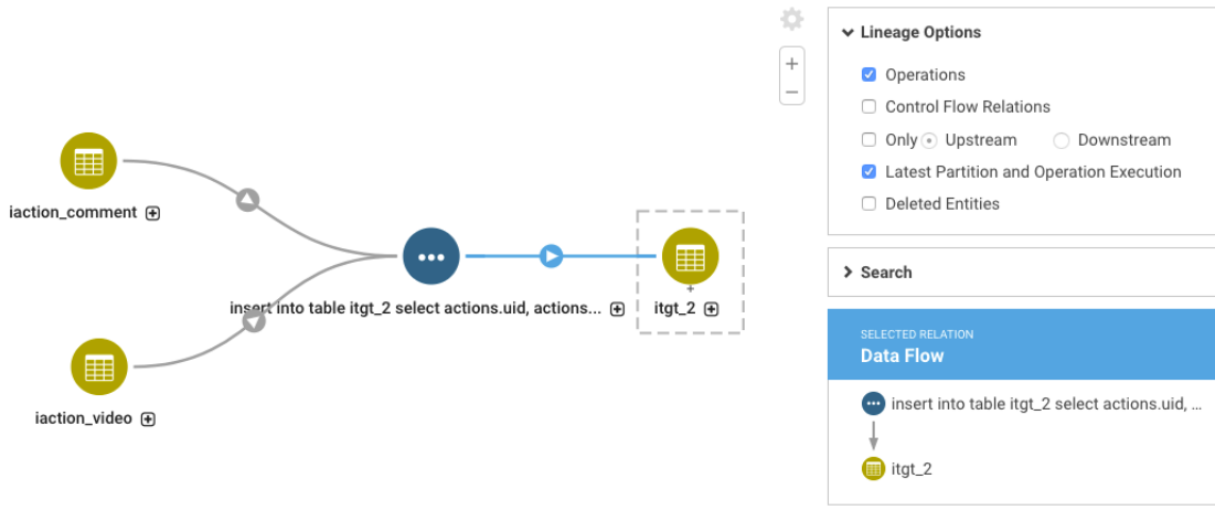
Figure 1: Impala Lineage
