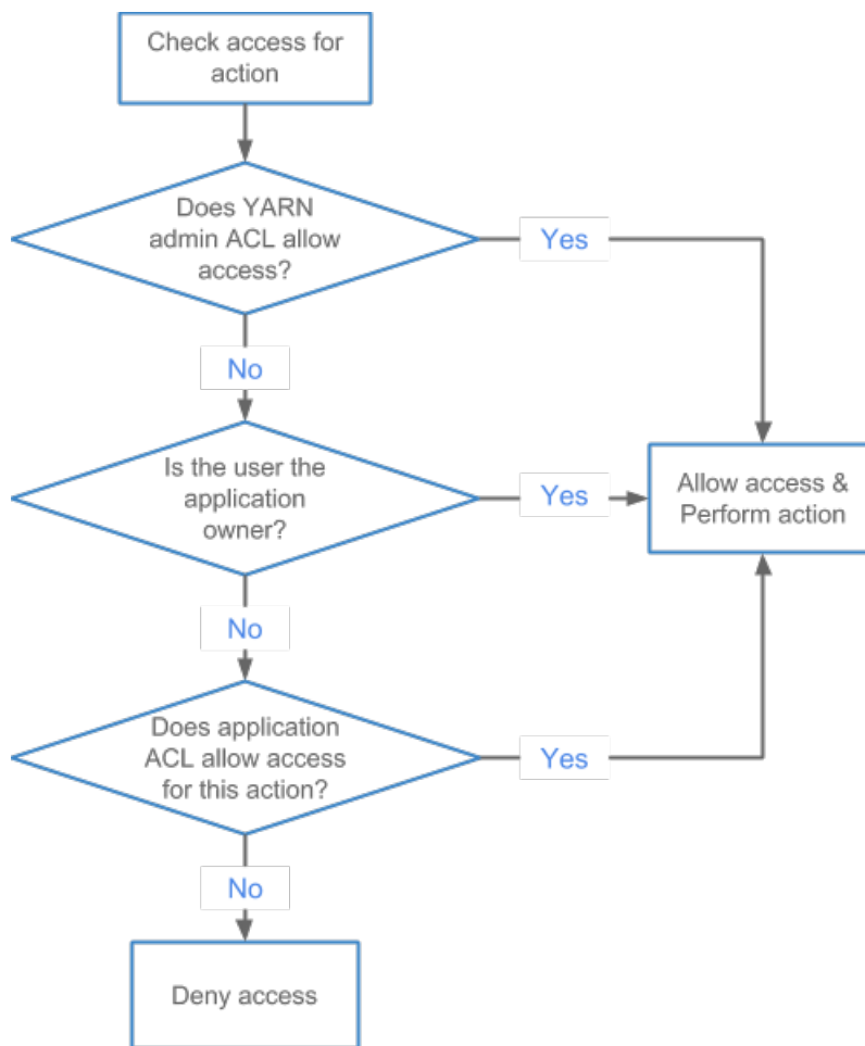
Figure 7: Application ACL Evaluation Flow
