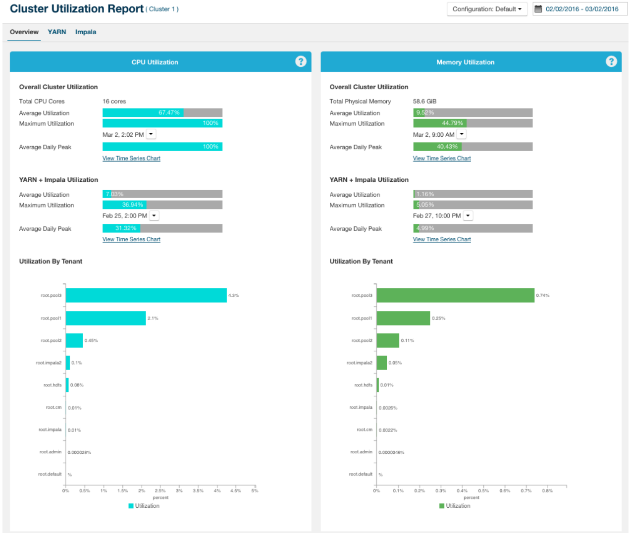
Figure 13: Cluster Utilization Report Overview Tab
